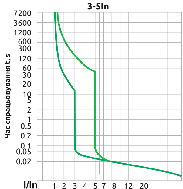
FMC3/3U (75-250A)
