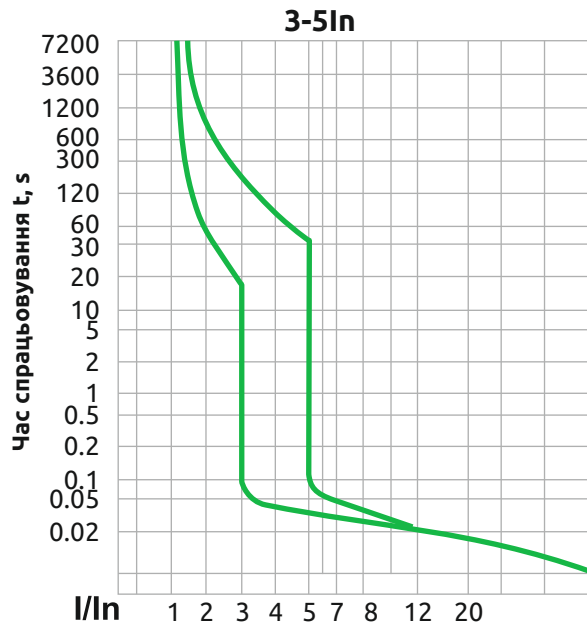
FMC3/3U (32-63A)
