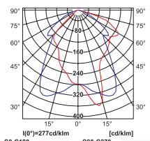
ADAMO MTH-400/A
