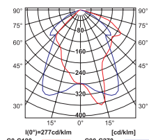
ADAMO MTH-250/A
