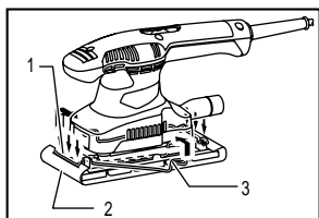
1. Clamping part 2. Abrasive paper 3. Clamp lever
