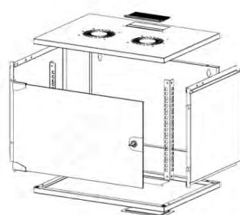
EXPLODED VIEW
