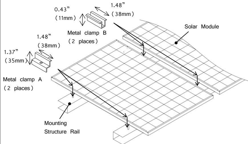
Figure 10-1 Installation A
