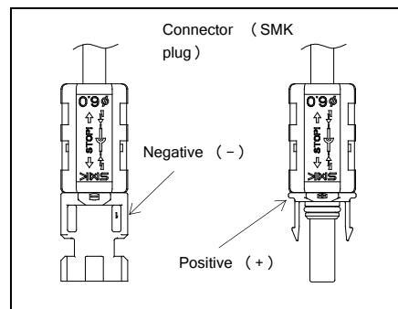
Figure 3: Configuration of Junction Box
