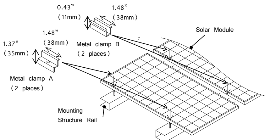
Figure 2-1 Installation A
