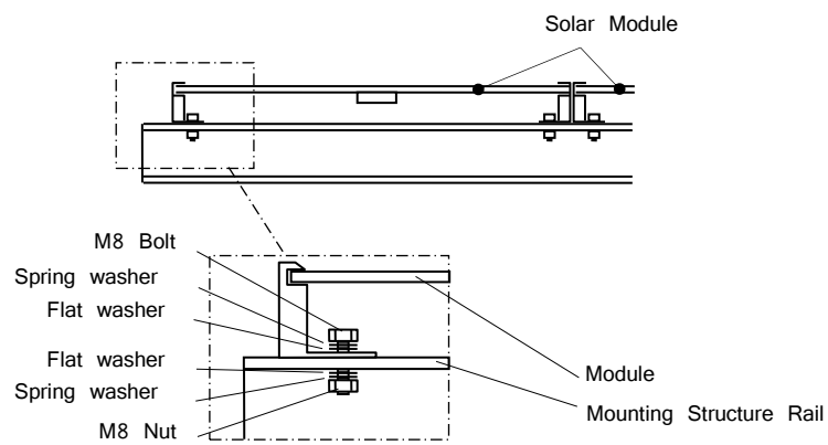
Figure 10-2 Installation B
