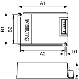
HID-PVe C 35 /S CDM 220-240V 50/60Hz
