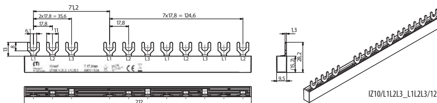
IZ10/L1L2L3NL1/NL/2NL3/N/12
