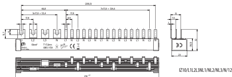
IZ10/L1L2L3N-L1NL2NL3N/12
