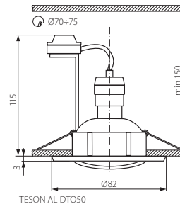
TESON AL-DT050
