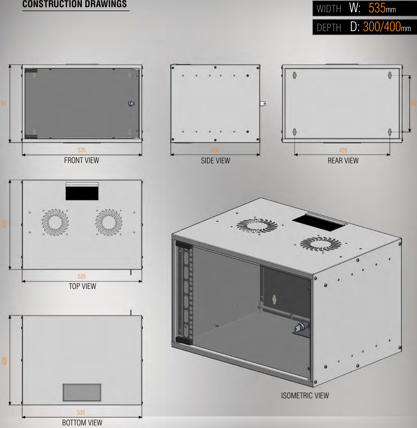
MR. SOHO 19" WALL TYPE CABINETS W=535mm D=300mm / 400mm
