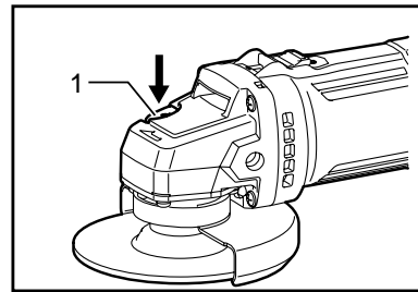
1. Shaft lock
