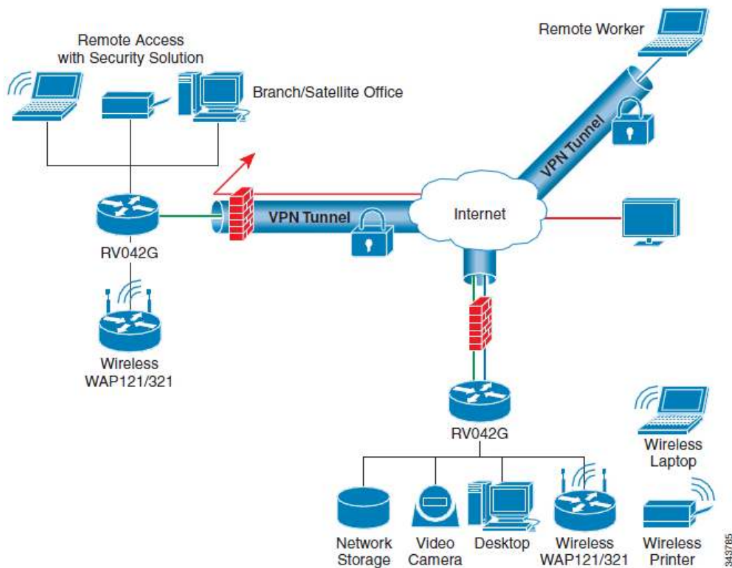
Figure 3. Typical Configuration
