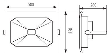
ANTRA LED200W
