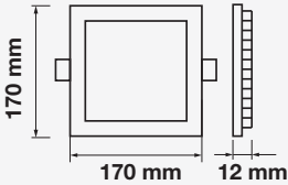
Cutting Size: 160x160mm
