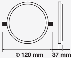
Cutting Size: ø 95 mm
