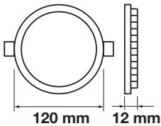
Cutting Size: \varnothing 110mm
