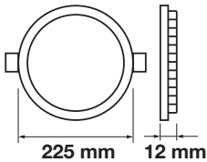
Cutting Size: \varnothing 210mm
