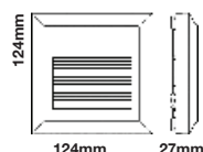
Step Light - IP65
