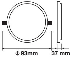
Cutting Size: ø 72 mm
