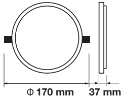
Cutting Size: ø 140 mm
