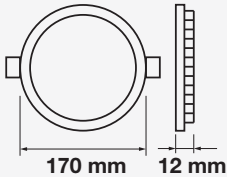
Cutting Size: \varnothing 160mm
