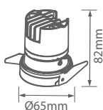
Cutting Size Ø55mm
