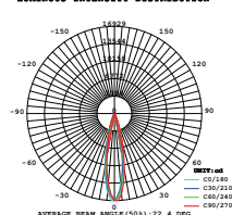
LUMINOUS INTENSITY DISTRIBUTION
