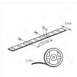
LEDS-P 10W/M IP00 WW
