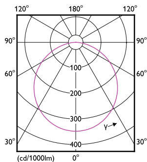
Downlight DN027B LED9 NW L125 SQ
